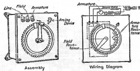
FIG. 94.—Non-automatic starting and speed-adjusting rheostat.
