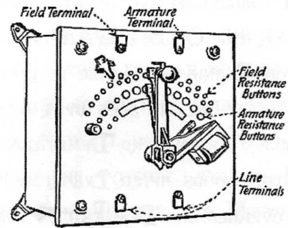
FIG. 102.—Starting and speed-adjusting rheostat.
